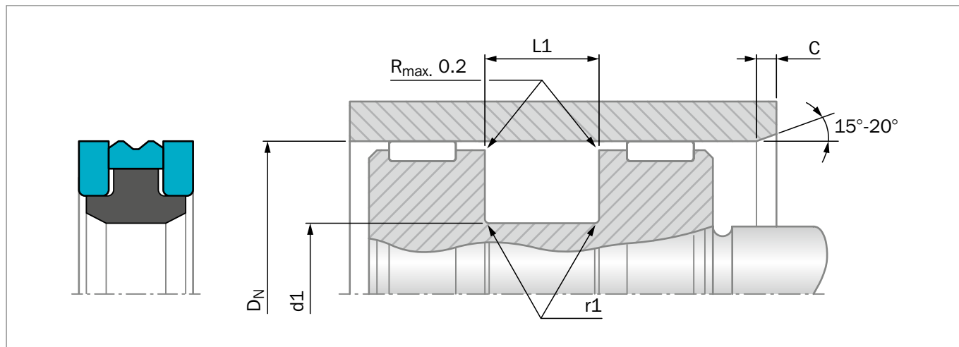
Figure 147: Installation Drawing
