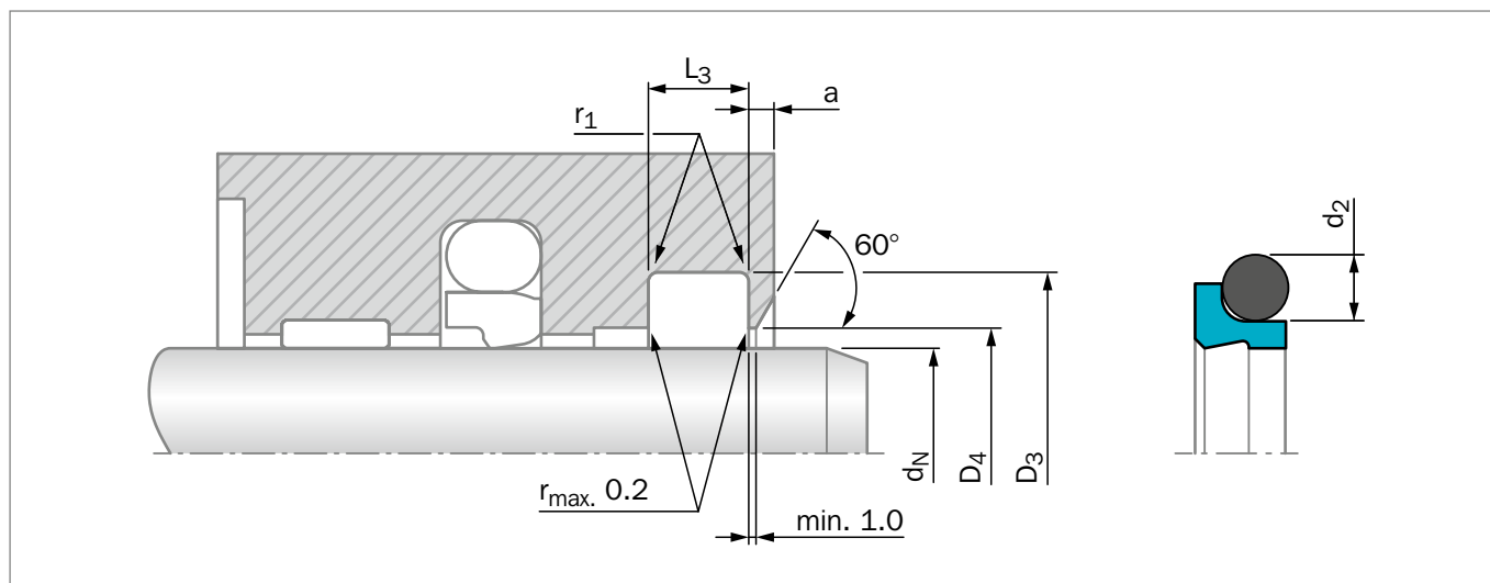
Figure 161: Installation Drawing
