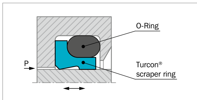
Figure 160: Turcon® Excluder® 2
