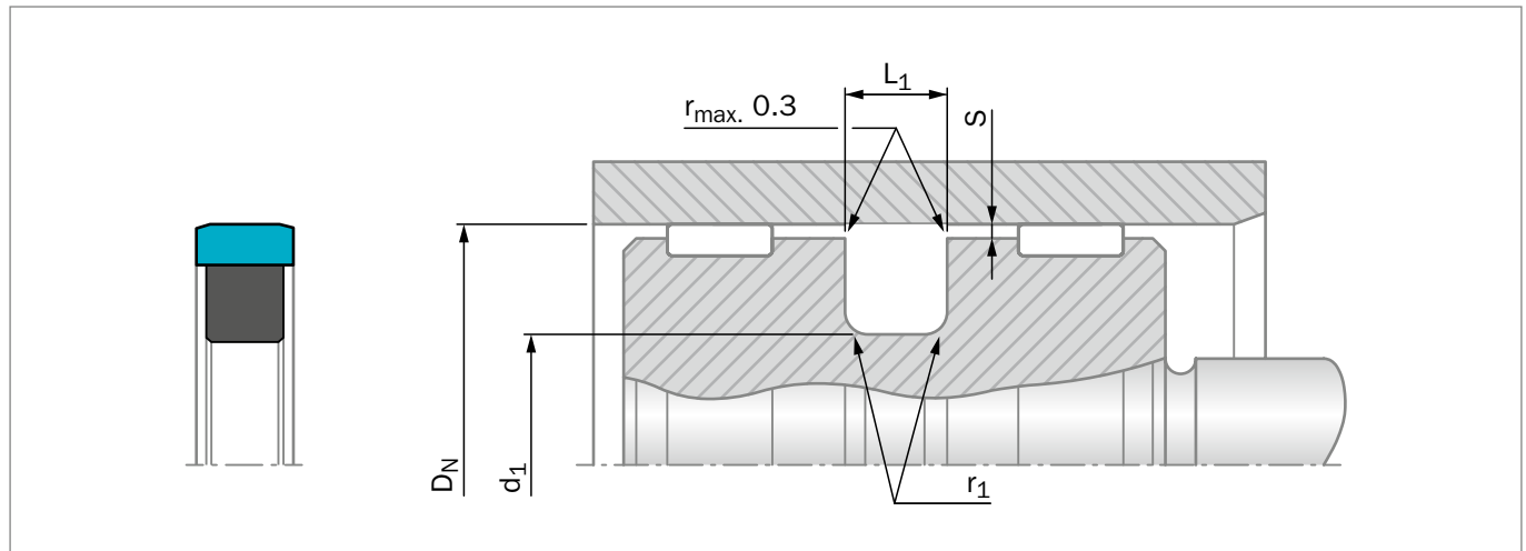
Figure 115: Installation Drawing
