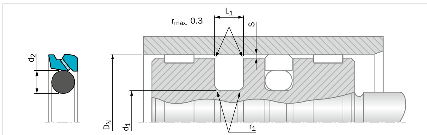
Figure 124: Installation Drawing
