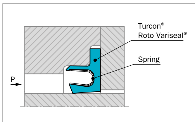
Figure 146: Turcon® Roto Variseal®
