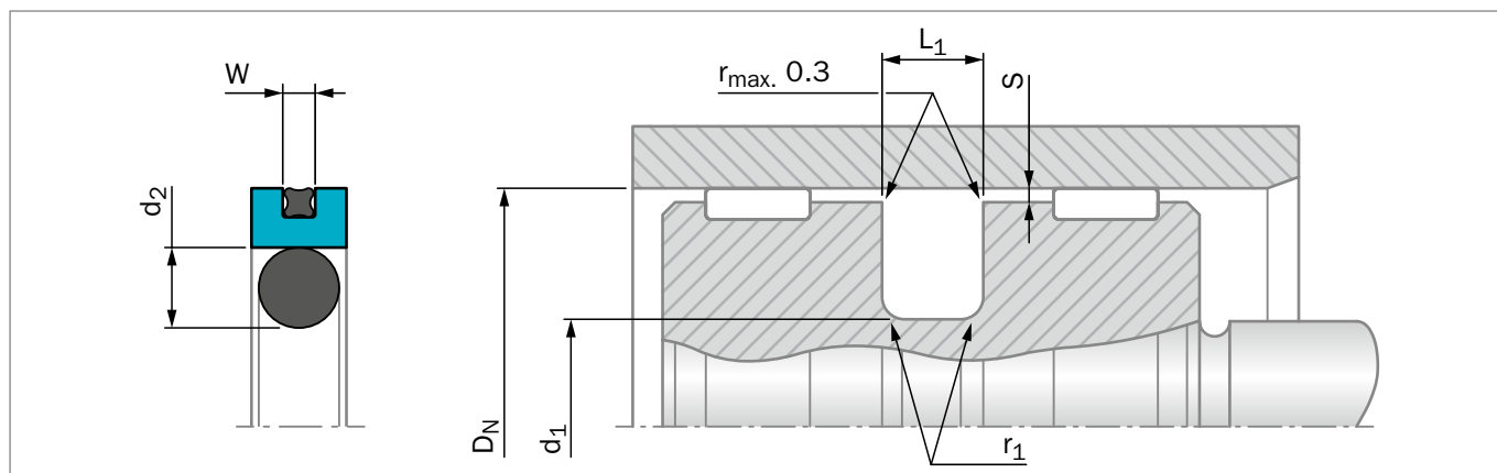
Figure 119: Installation Drawing
