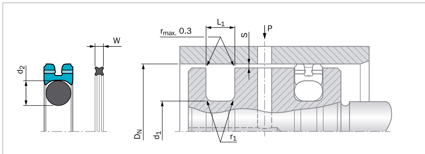
Figure 139: Installation Drawing
