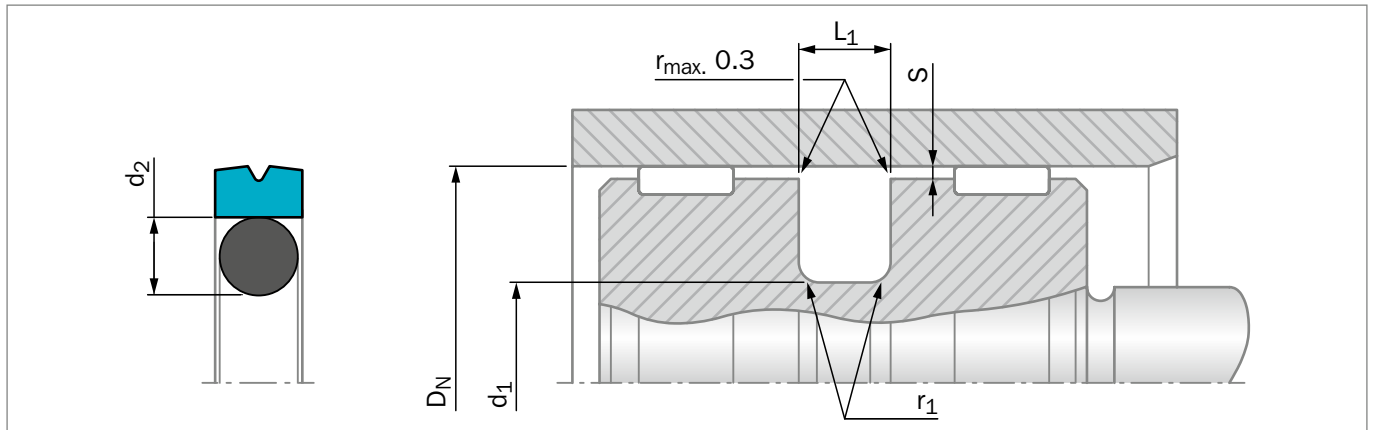
Figure 110: Installation Drawing
