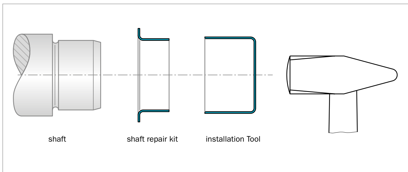
Figure 72: Installation sequence
