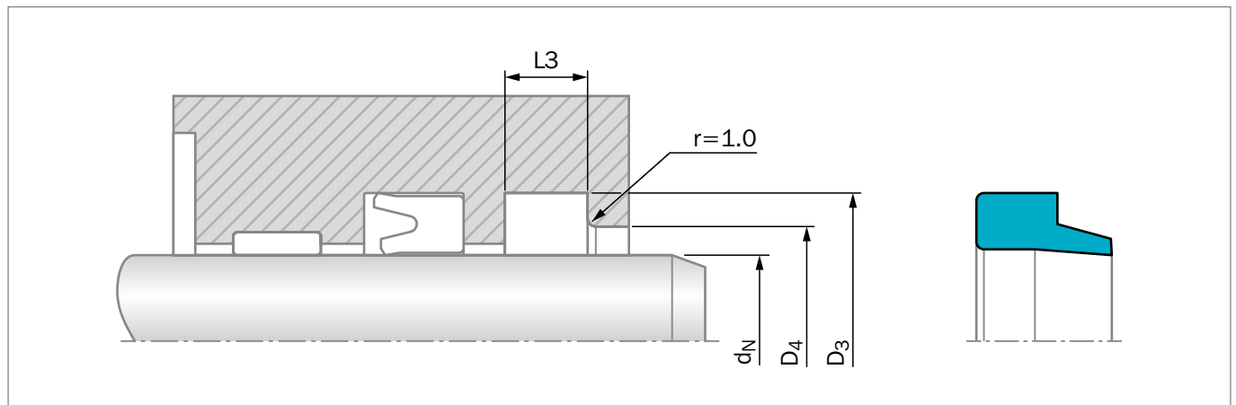
Figure 191: Installation Drawing
