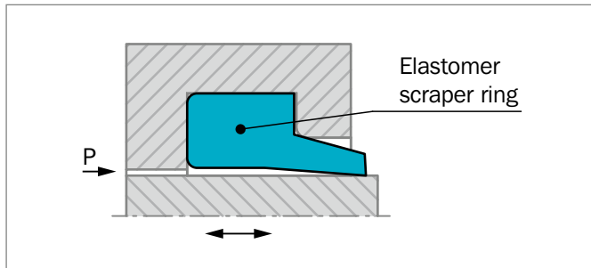
Figure 190: Scraper WRM
