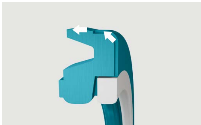
Figure 59: Venting path
