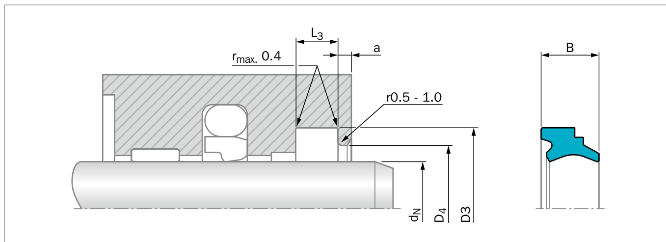
Figure 184: Installation Drawing
