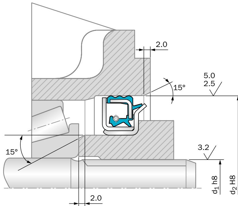
Figure 60: System 5000 in pinion application
