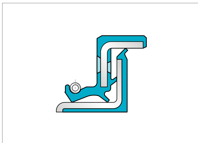
Figure 66: "Hygienic design" APJ for food applications
