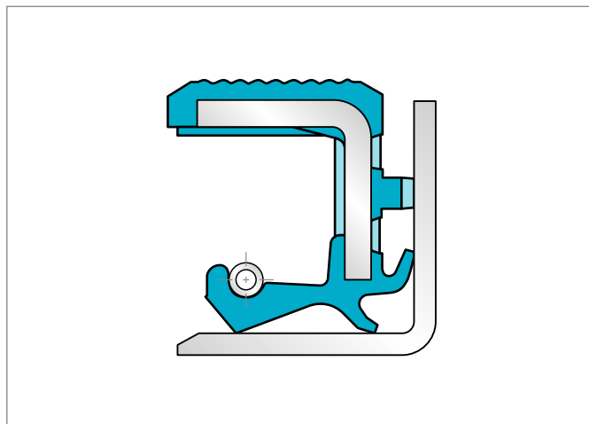
Figure 65: APJ for corrosive applications
