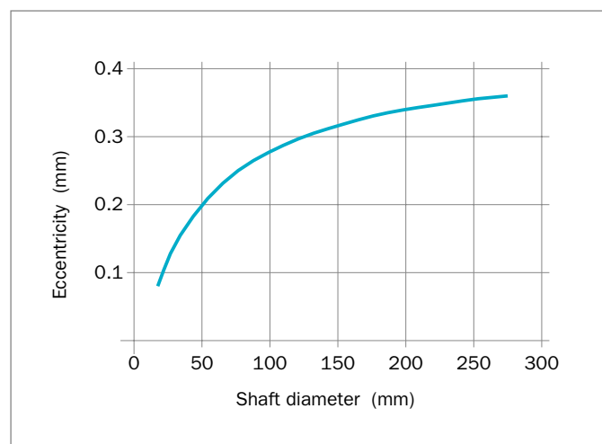
Figure 62: Permissible eccentricity
