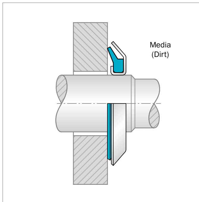
Figure 89: Installation Drawing
