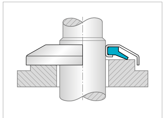
Figure 88: Vertical installation
