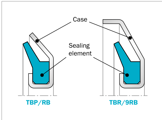
Figure 86: GAMMA Seal types
