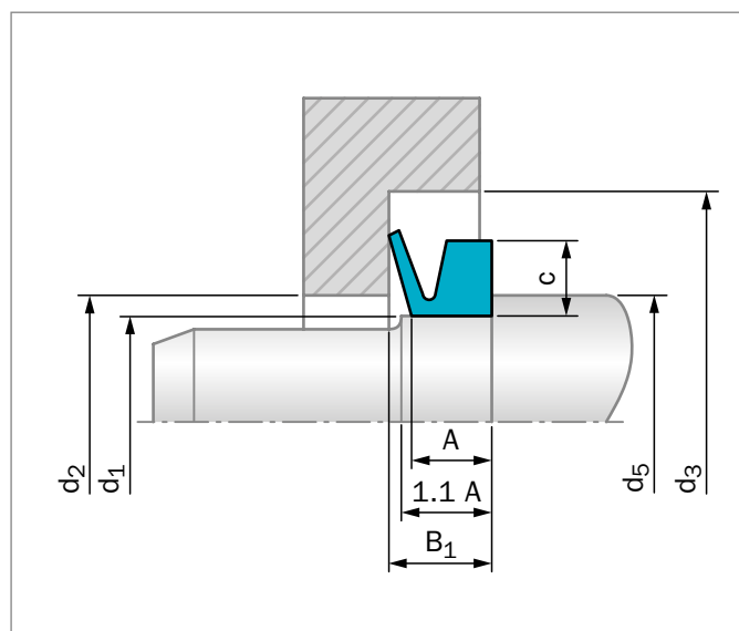
Figure 78: Axial support
