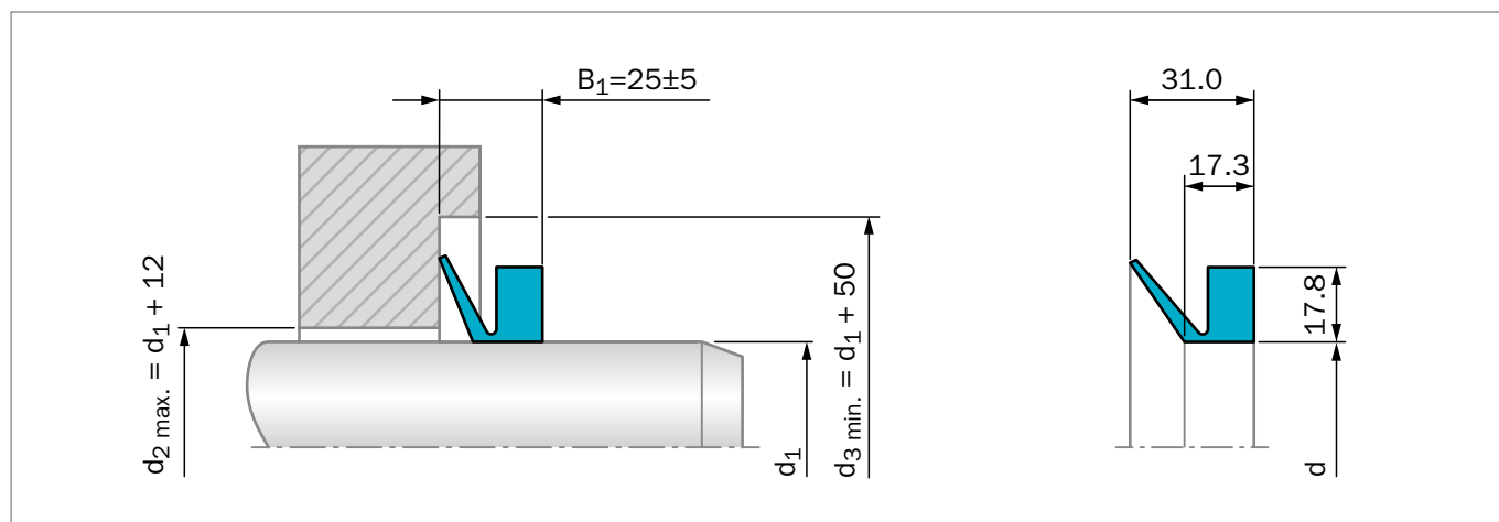
Figure 85: Installation Drawing
