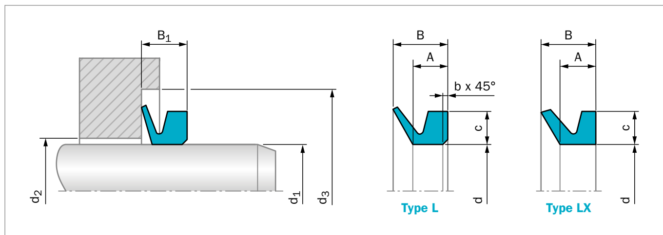
Figure 83: Installation Drawing
