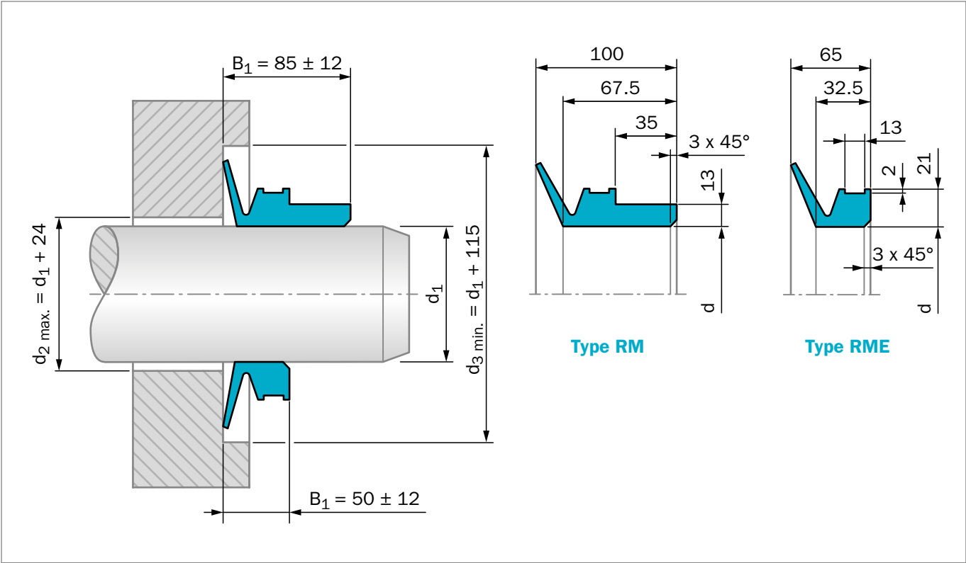
Figure 84: Installation Drawing
