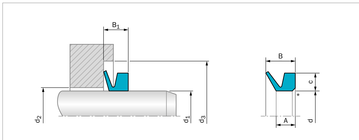
Figure 81: Installation Drawing
