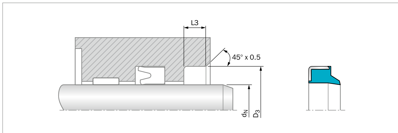
Figure 197: Installation Drawing
