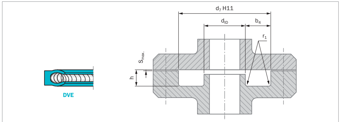
Figure 26: Installation drawing
