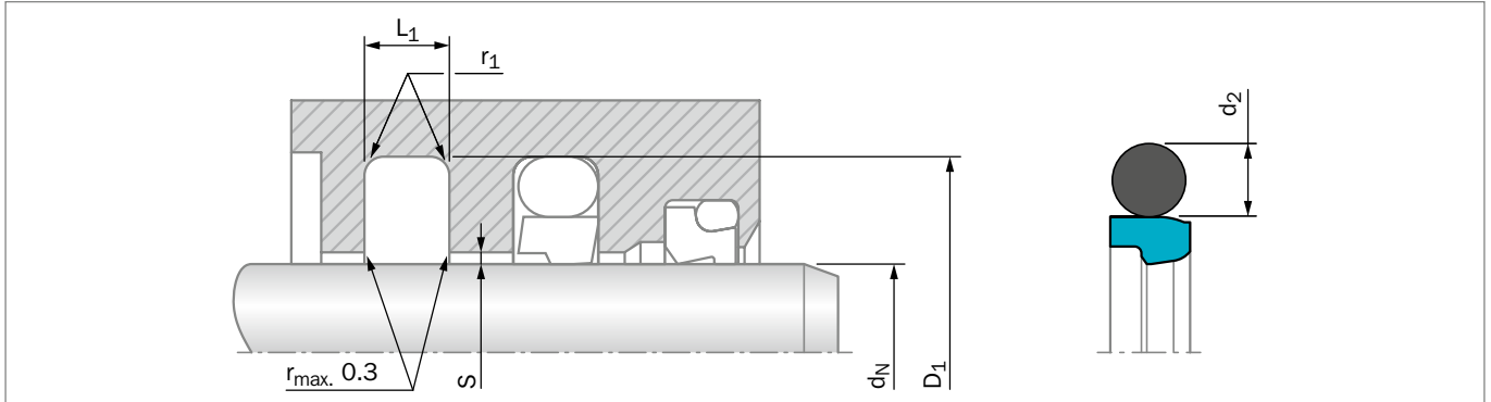
Figure 22: Installation Drawing
