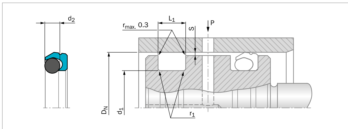
Figure 155: Installation Drawing
