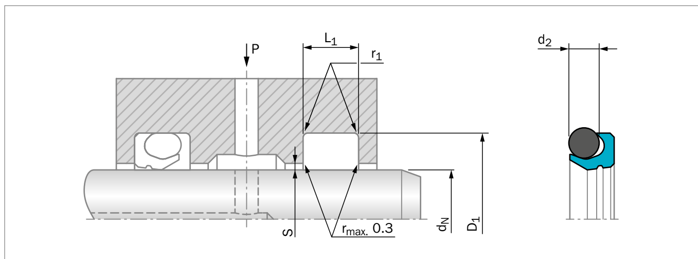
Figure 154: Installation Drawing
