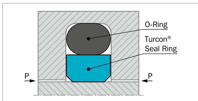
Figure 70: Turcon® Glyd Ring®
