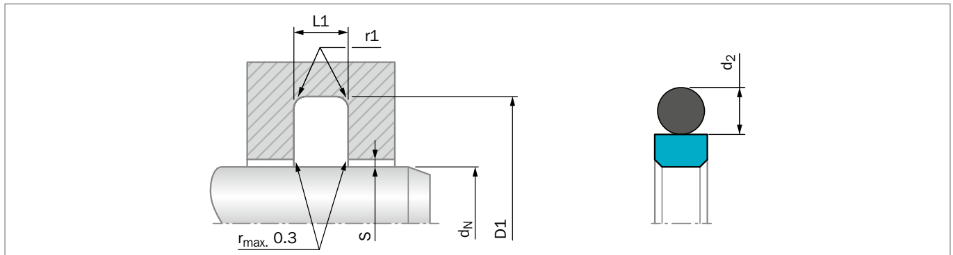
Figure 72: Installation Drawing
