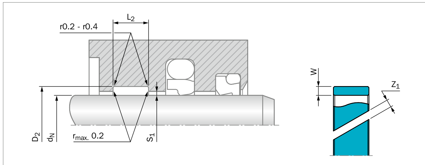
Figure 222: Installation Drawing
