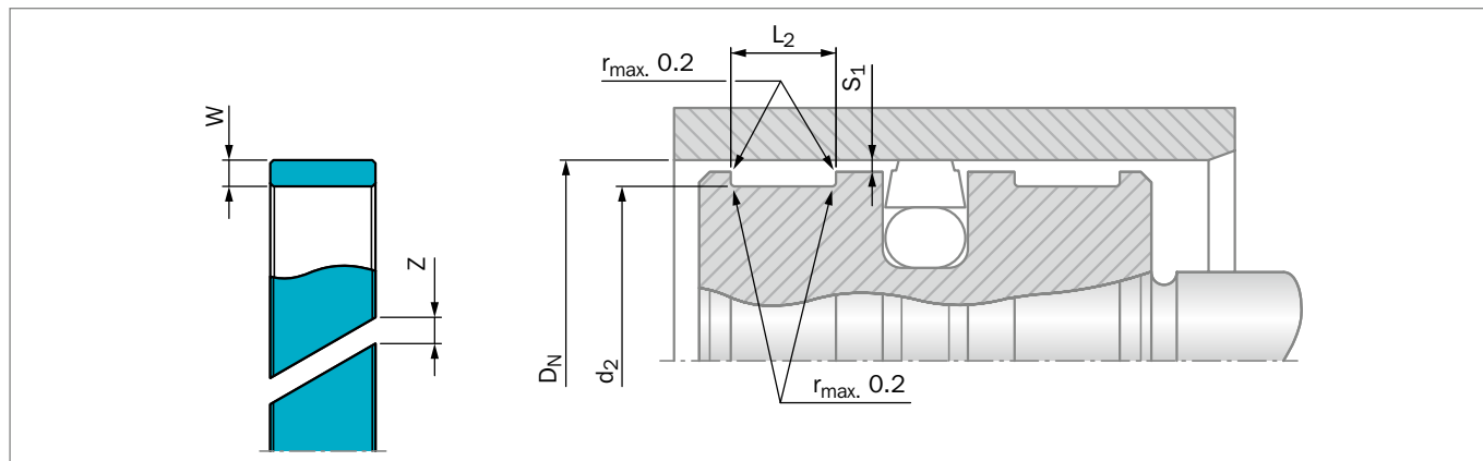
Figure 213: Installation Drawing
