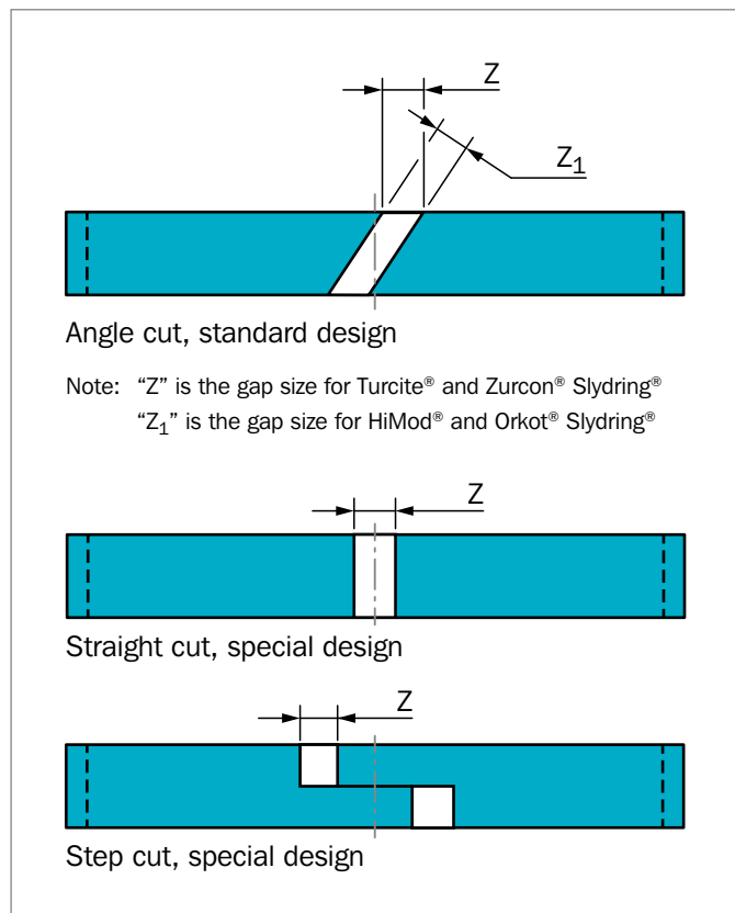
Figure 205: Type of cut
