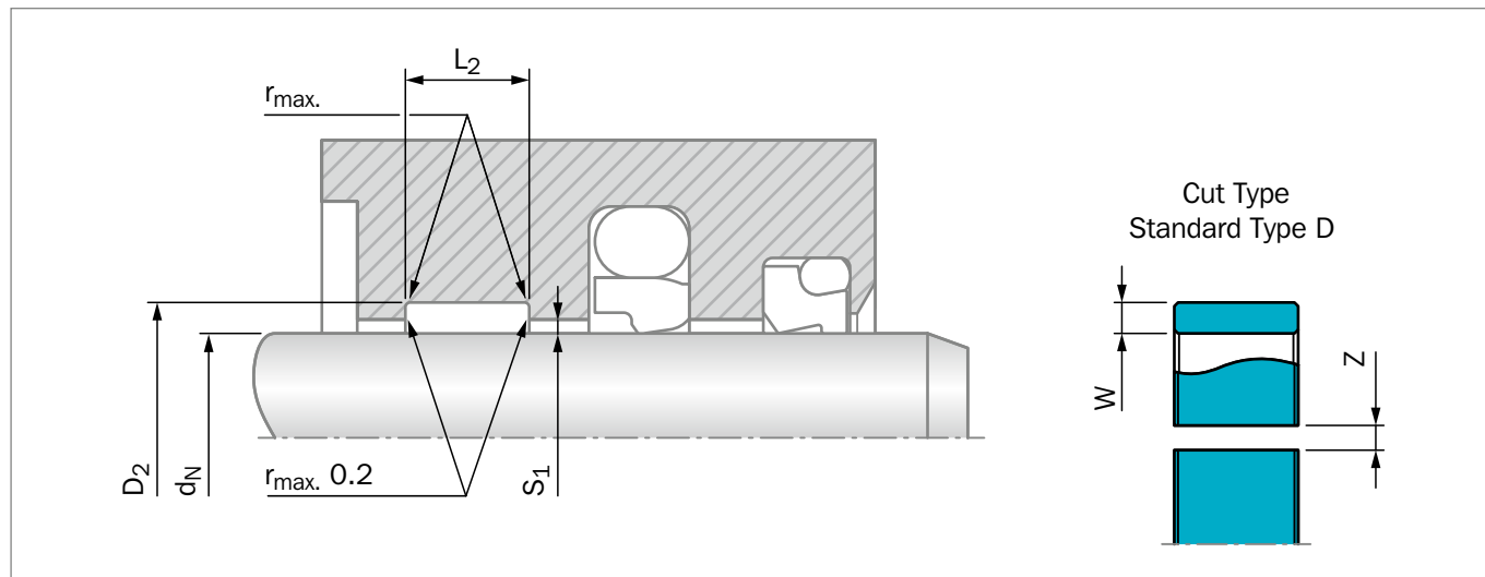
Figure 218: Installation Drawing
