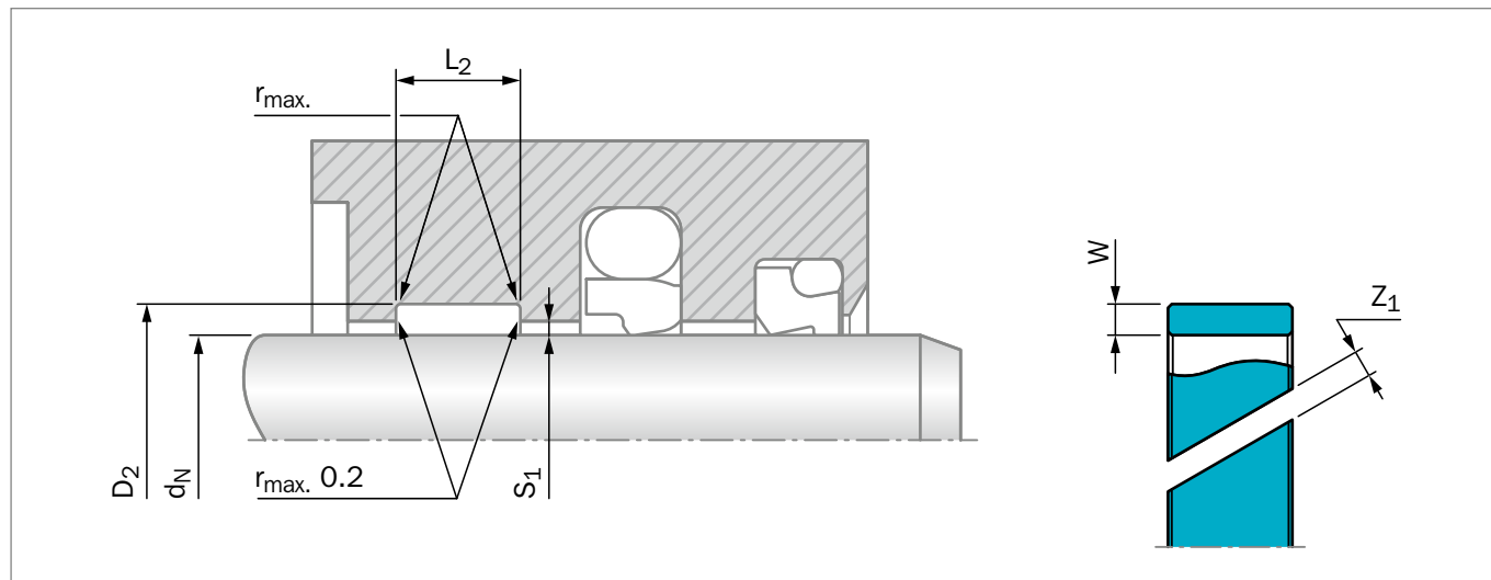
Figure 217: Installation Drawing
