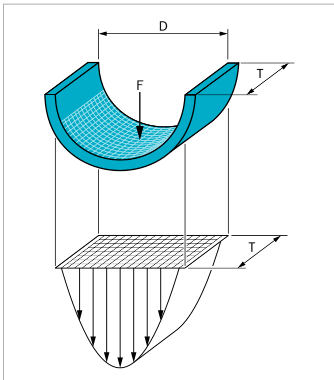
Figure 206: Load distribution
