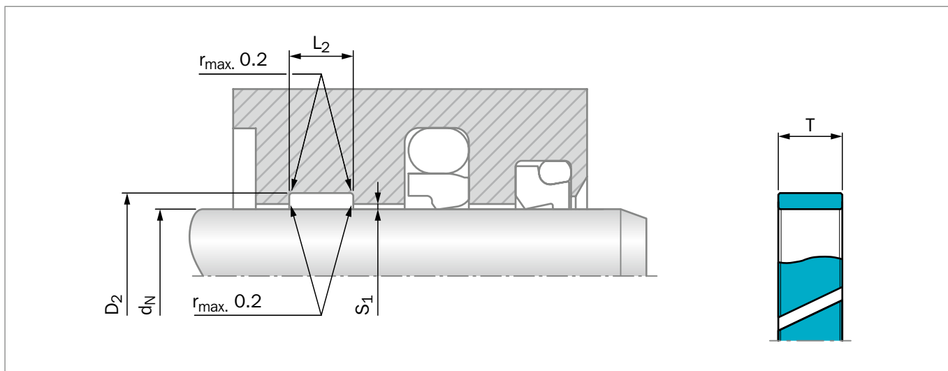
Figure 208: Rod guide
