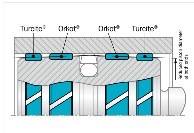
Figure 219: Arrangement of the Slydring® on the piston
