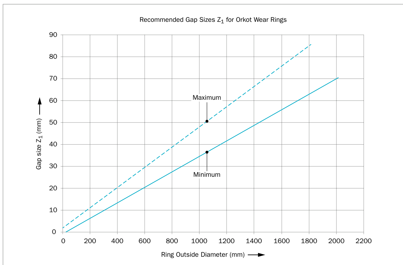
Figure 221: Recommended Gap Sizes Z_1 for Orkot Wear Ring
