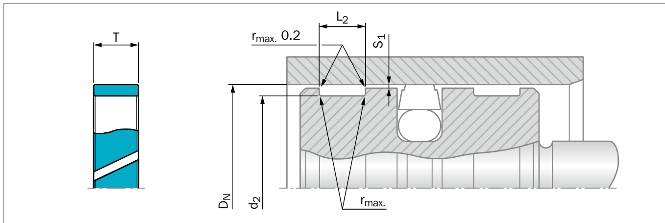
Figure 207: Piston guide
