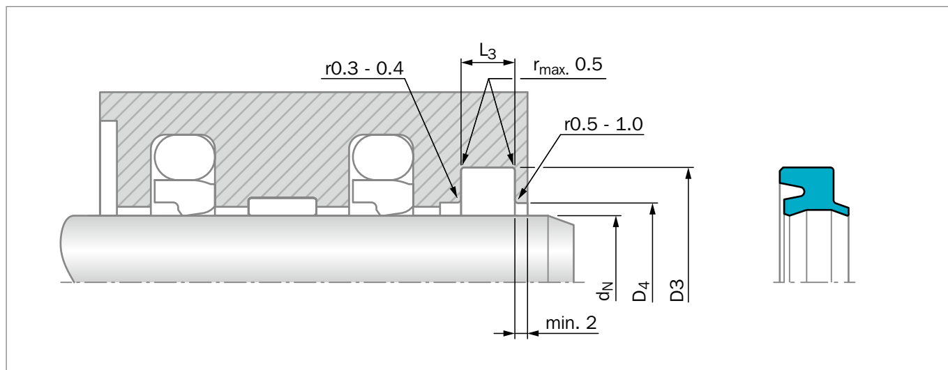
Figure 186: Installation Drawing
