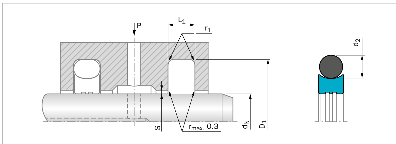
Figure 128: Installation Drawing
