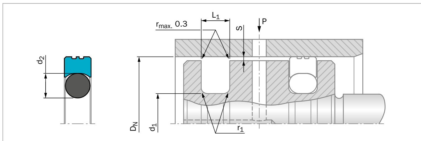
Figure 129: Installation Drawing
