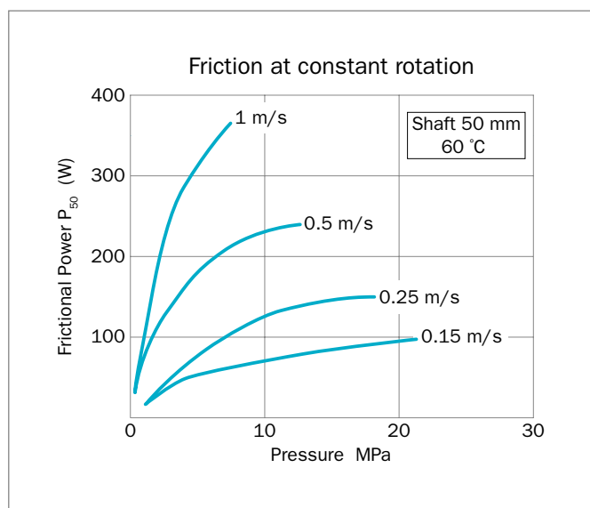
Figure 127: Frictional power for Turcon® Roto Glyd Ring®
