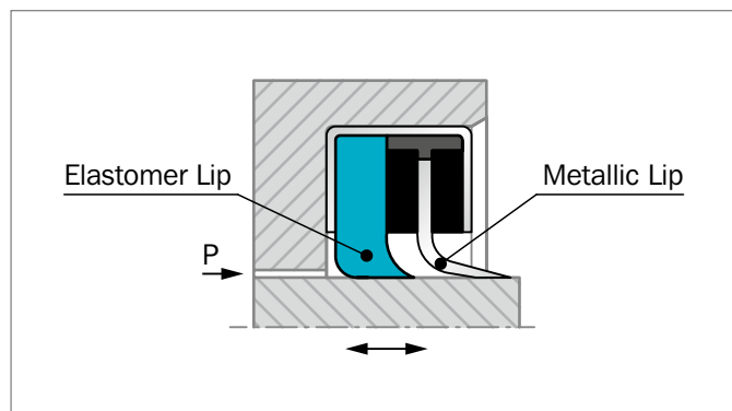
Figure 200: Metal Scraper
