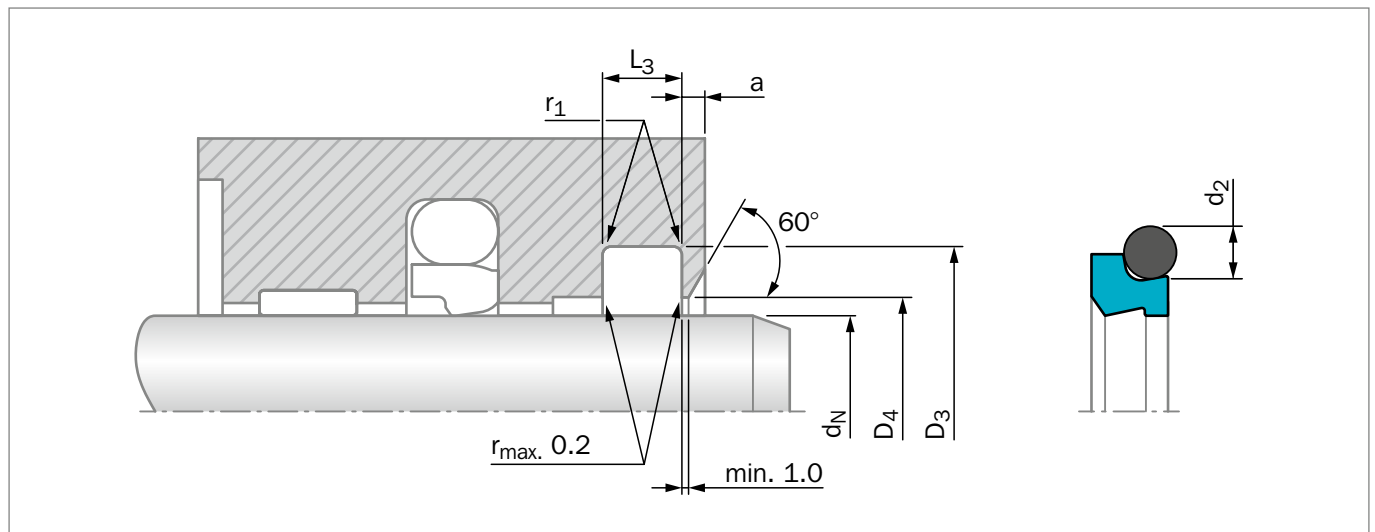
Figure 163: Installation Drawing
