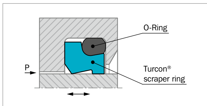
Figure 162: Turcon® Excluder® 5
