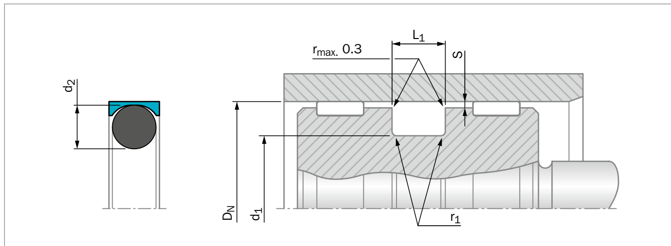
Figure 130: Installation Drawing
