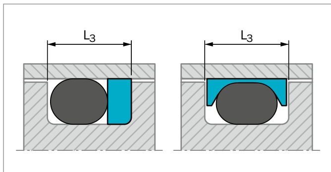
Figure 131: Groove width
